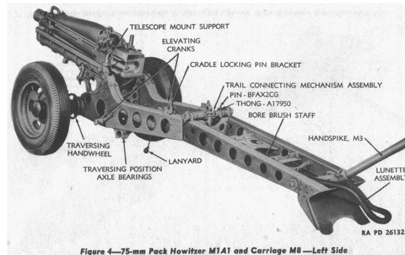
Figure 4—75-mm Pack Howitzer M1A1 and Carriage M8—Left Side
